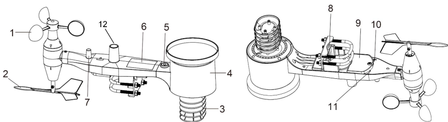
Figure 2: Sensor assembly components
