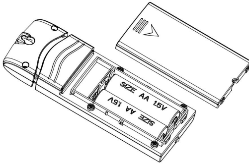
Figure 12: Indoor sensor battery installation
