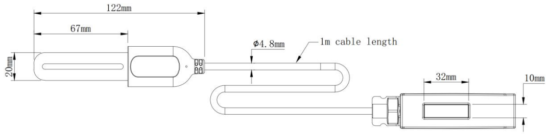
Figure 10: Main View
